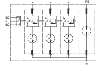
SCHEMATIC 6
