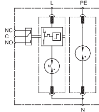
SCHEMATIC 5
