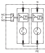
SCHEMATIC 5
