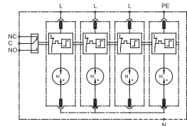
SCHEMATIC 4
