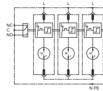
SCHEMATIC 6
